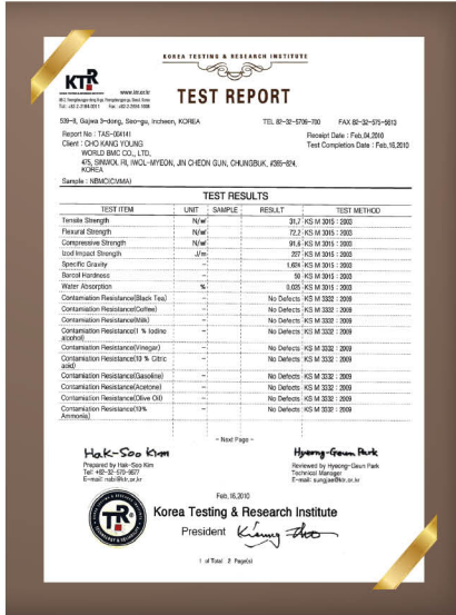
Mechanical Properties
